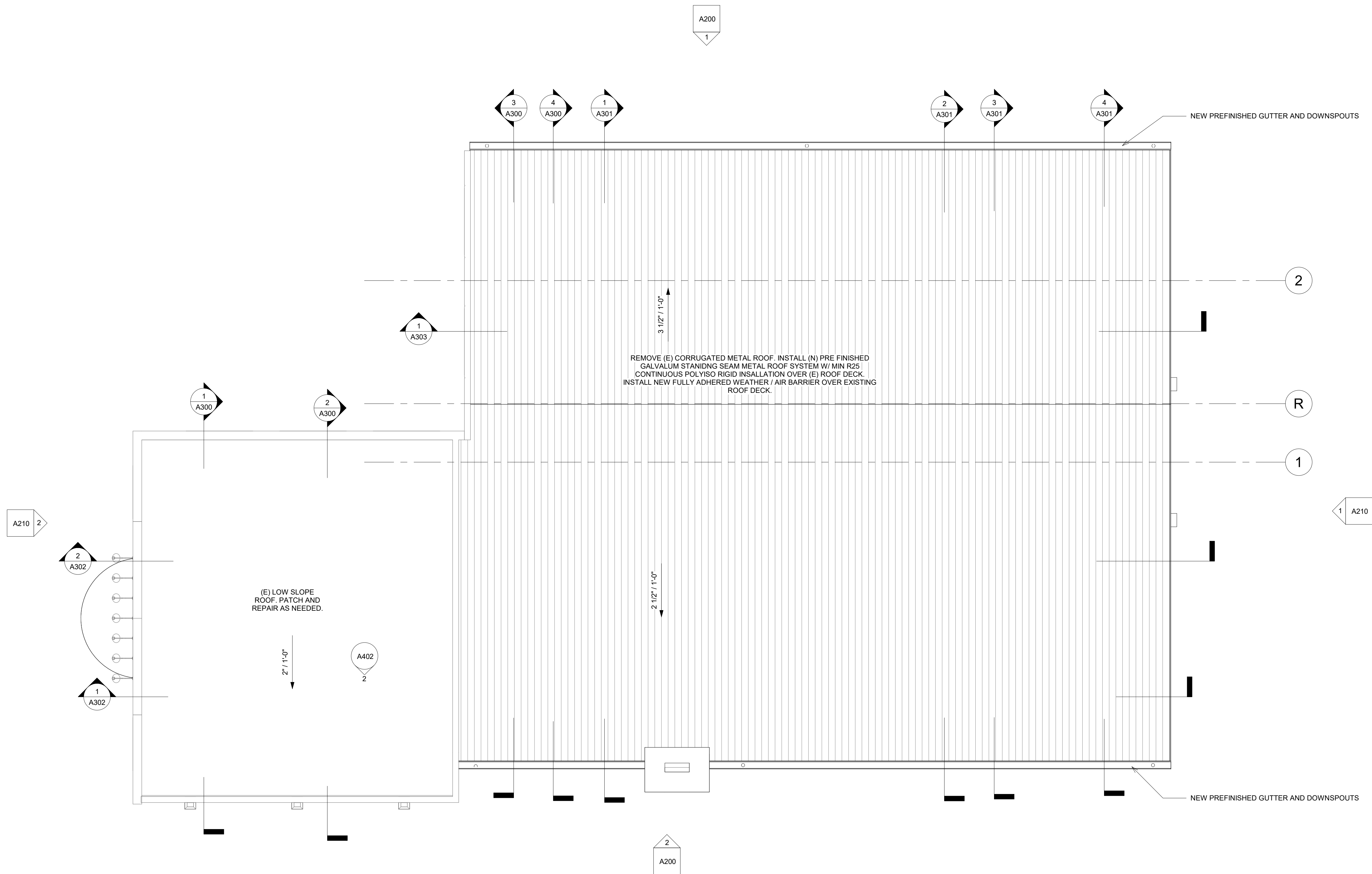
1 ROOF PLAN 1/4" = 1'-0"
