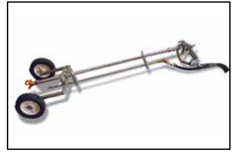
Apply paint and beads simultaneously with pole gun attachment and 25' hoses
